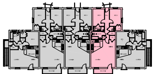
FIRST FLOOR 1:500 @ A4
