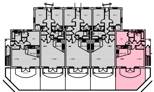
GROUND FLOOR 1:500 @ A4
