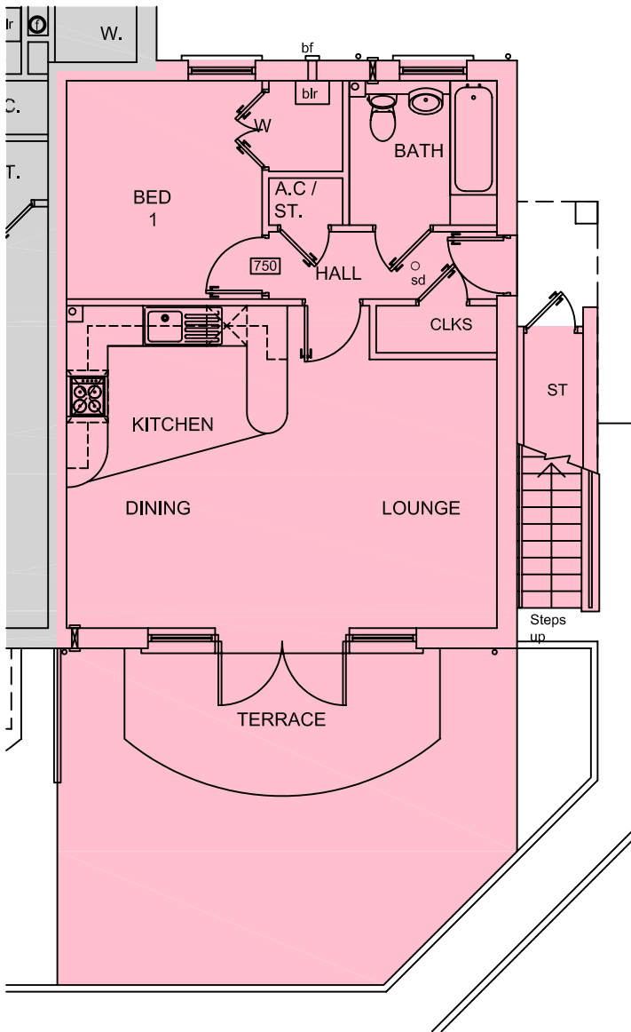
GROUND FLOOR 1:100 @ A4
