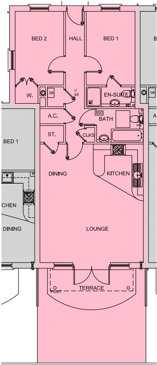
GROUND FLOOR 1:100 @ A4
